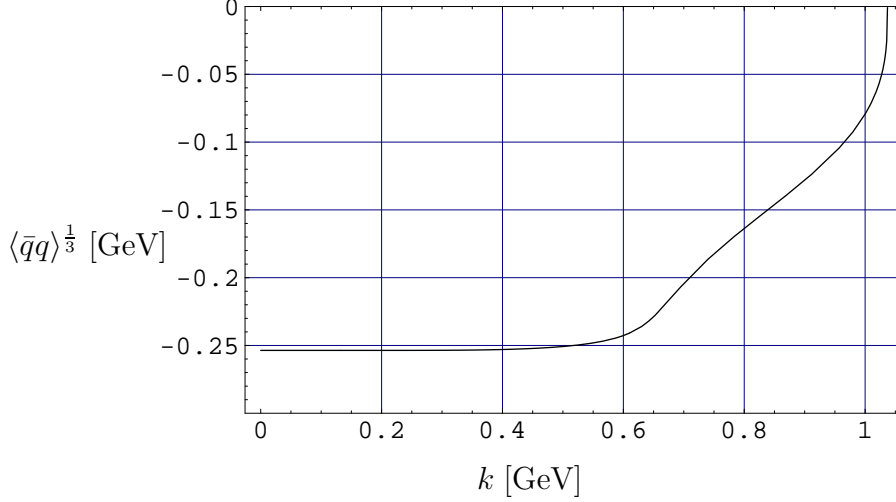
Figure 1: The evolution of the chiral quark condensate as a function of the renormalization scale k with an explicit symmetry breaking due to a current quark mass of m_q = 7 MeV.
